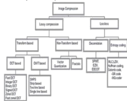
Figure 1.1. Image Compression Techniques
